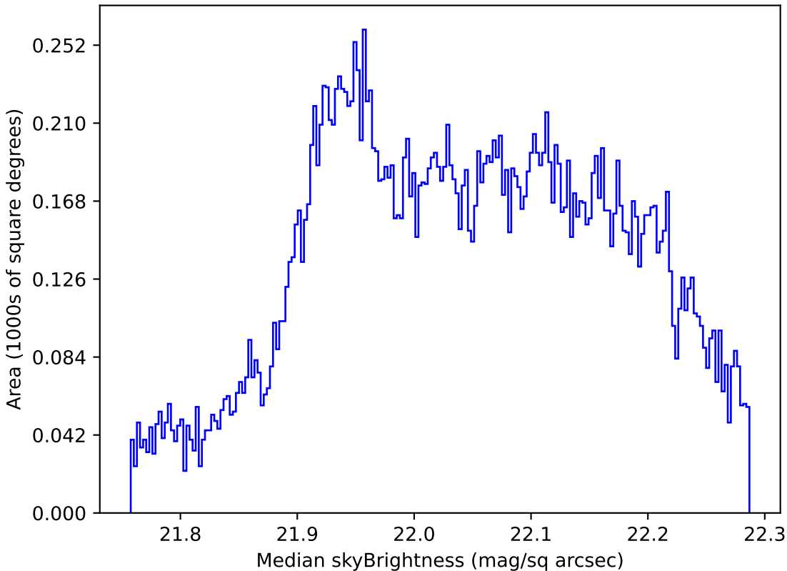
start_date_do90v3.4_10yrs All sky g band: Median skyBrightness
