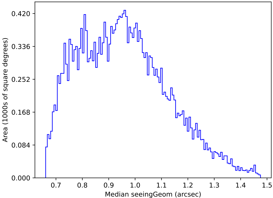
start_date_do90v3.4_10yrs Yr 1 g band: Median seeingGeom
