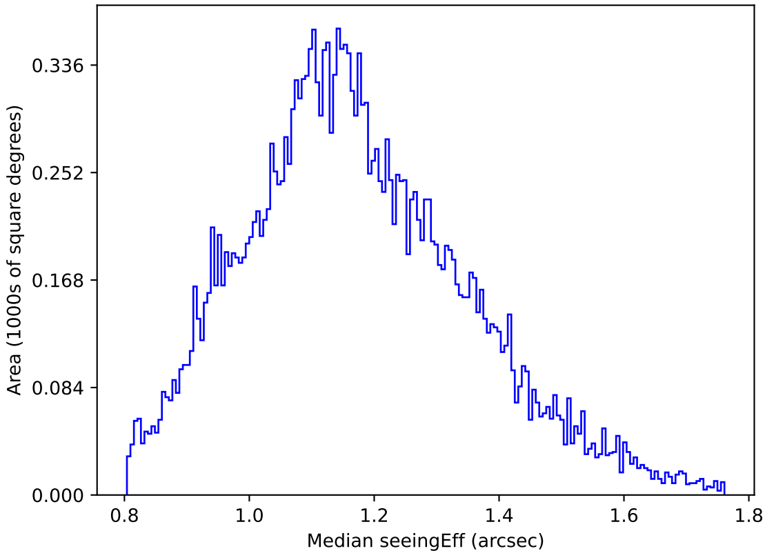
start_date_do90v3.4_10yrs Yr 1 u band: Median seeingEff
