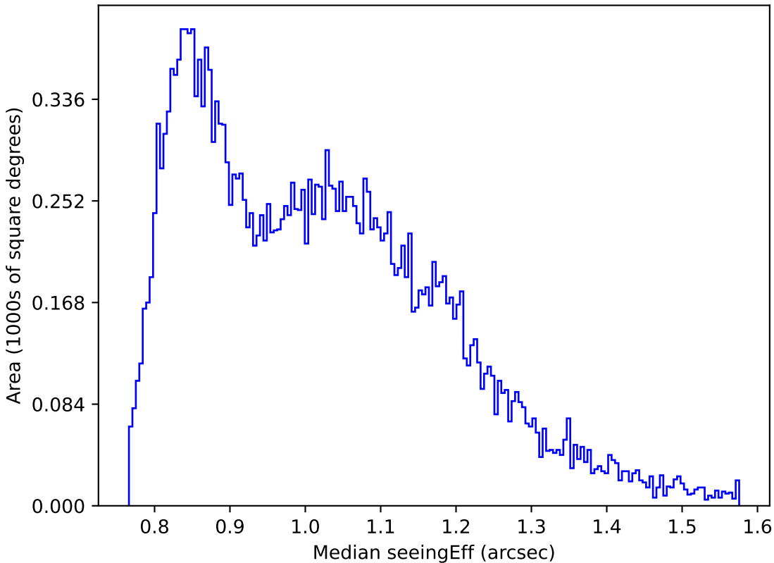
start_date_do90v3.4_10yrs Yr 1 r band: Median seeingEff
