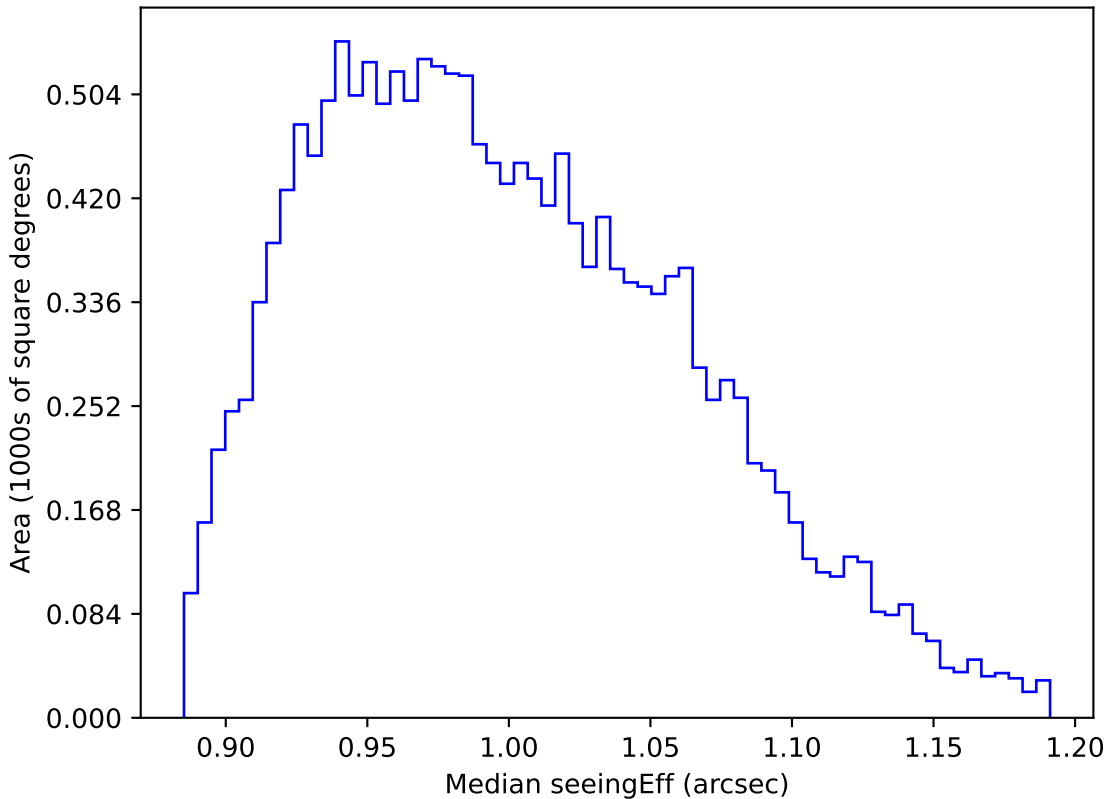
start_date_do90v3.4_10yrs WFD y band: Median seeingEff
