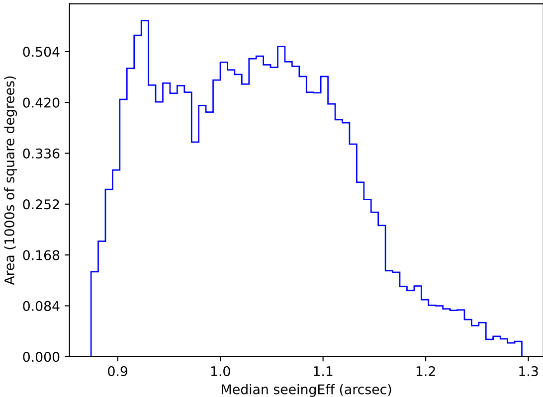
start_date_do90v3.4_10yrs WFD r band: Median seeingEff
