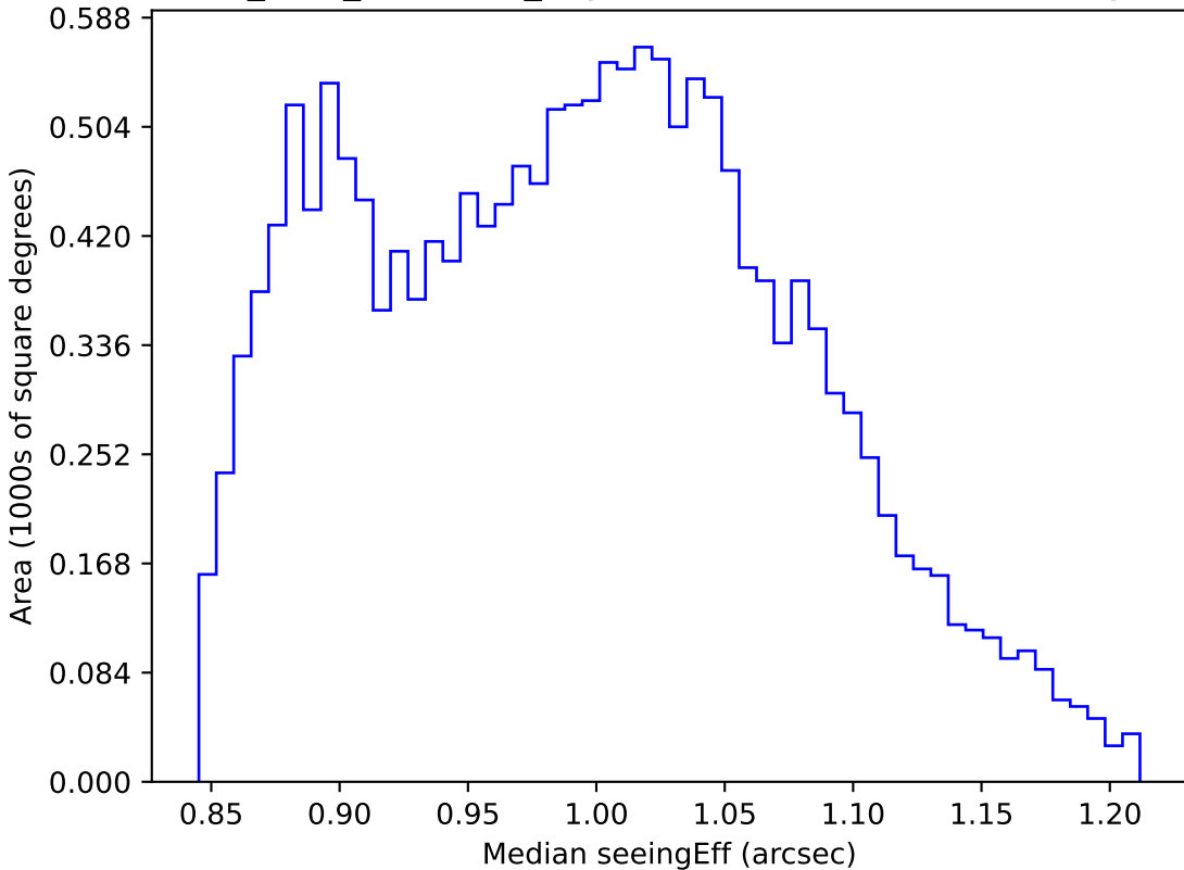
start_date_do90v3.4_10yrs WFD i band: Median seeingEff
