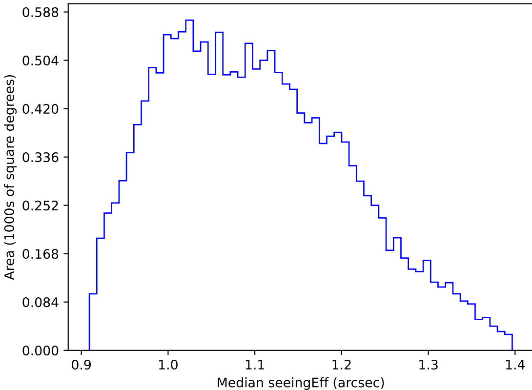
start_date_do90v3.4_10yrs WFD g band: Median seeingEff
