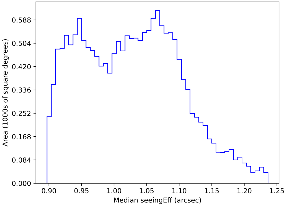
start_date_do90v3.4_10yrs WFD all bands: Median seeingEff
