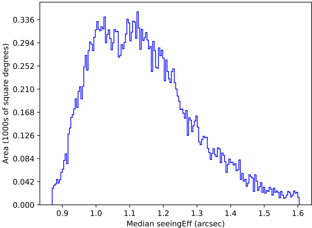
start_date_do90v3.4_10yrs All sky g band: Median seeingEff
