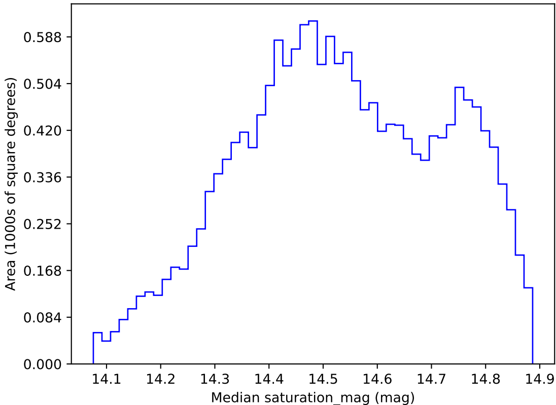
start_date_do90v3.4_10yrs WFD i band: Median saturation_mag
