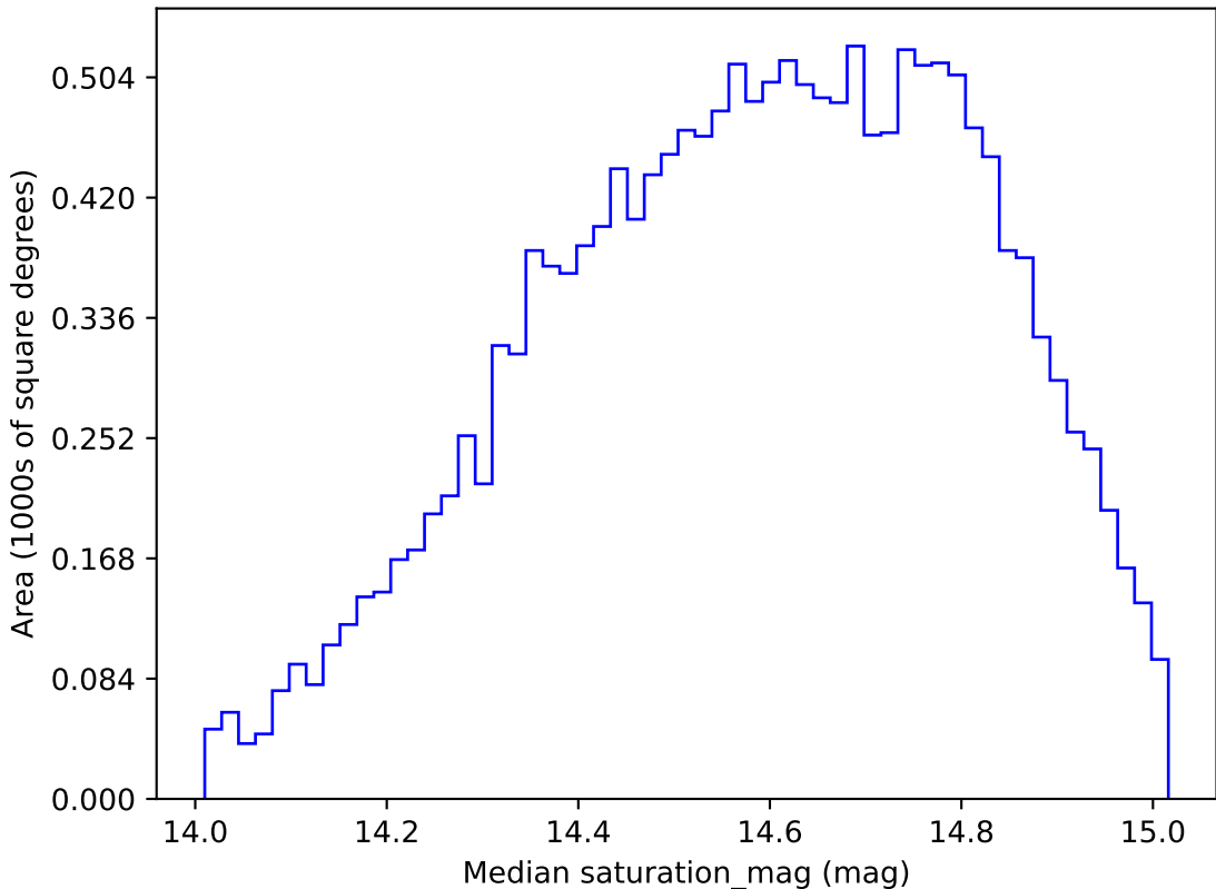
start_date_do90v3.4_10yrs WFD g band: Median saturation_mag
