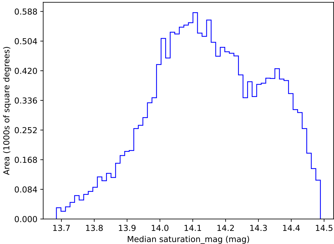
start_date_do90v3.4_10yrs WFD all bands: Median saturation_mag
