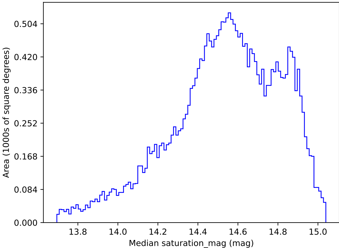
start_date_do90v3.4_10yrs All sky r band: Median saturation_mag
