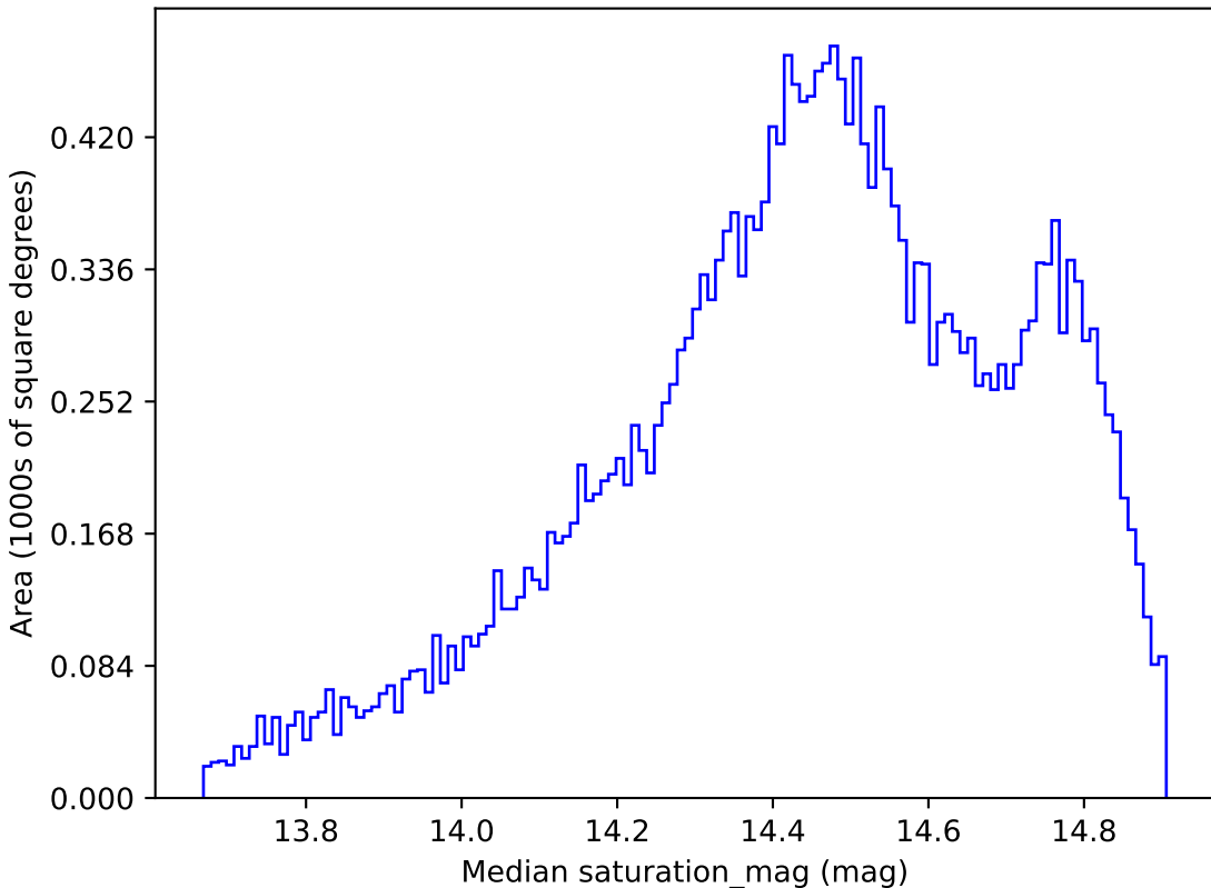
start_date_do90v3.4_10yrs All sky i band: Median saturation_mag
