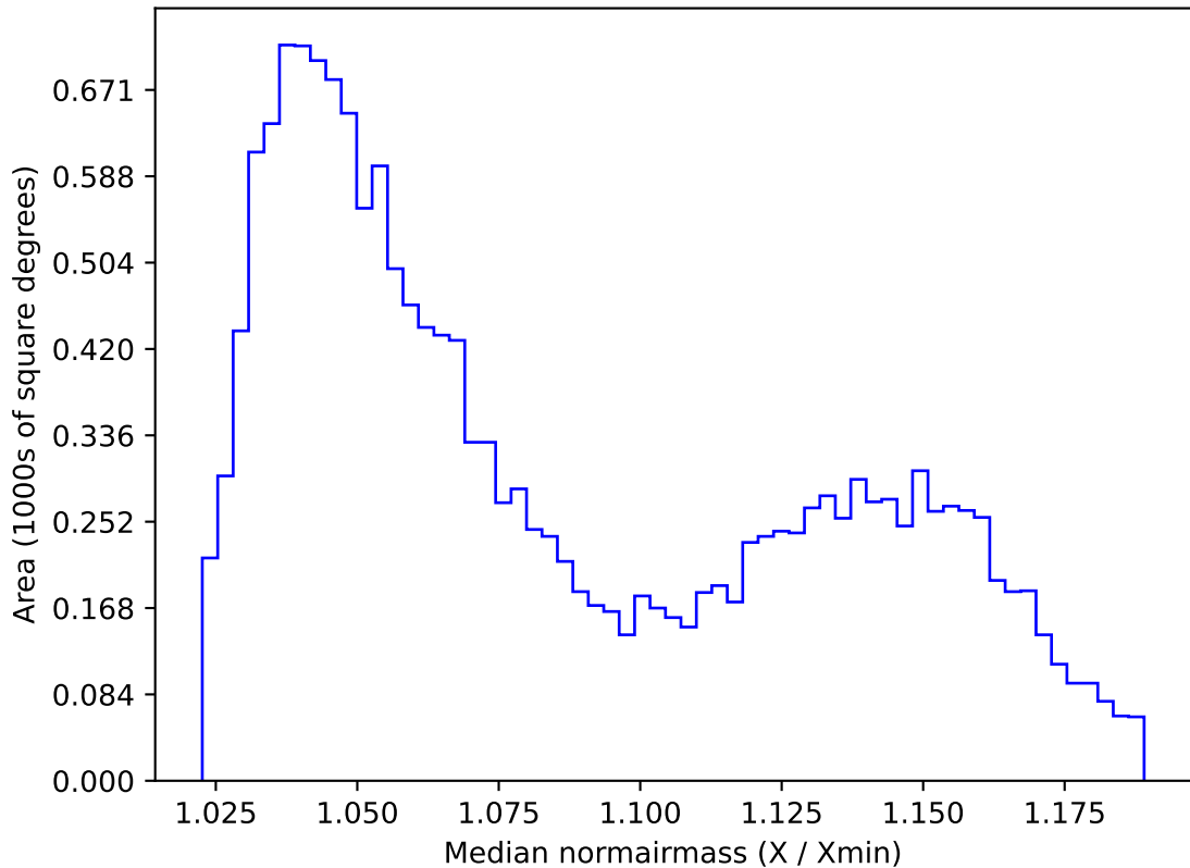
start_date_do90v3.4_10yrs WFD z band: Median normairmass
