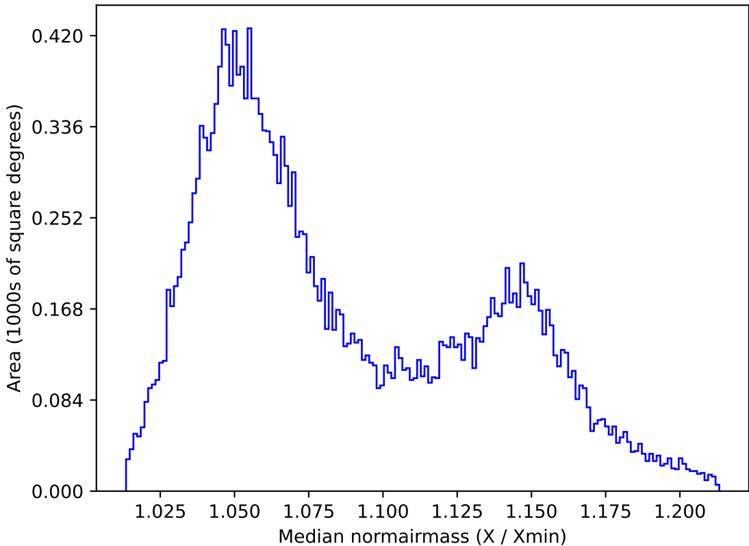
start_date_do90v3.4_10yrs All sky y band: Median normairmass
