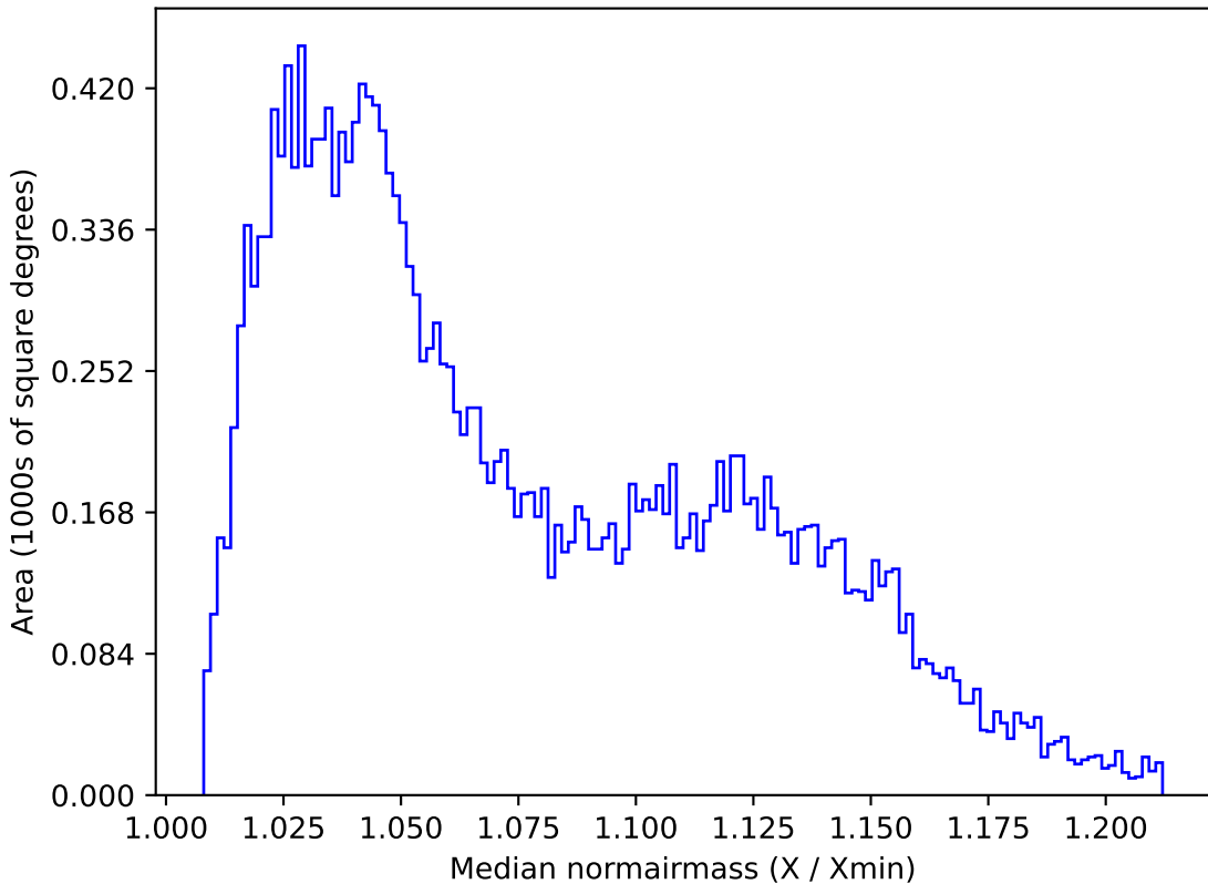
start_date_do90v3.4_10yrs All sky u band: Median normairmass
