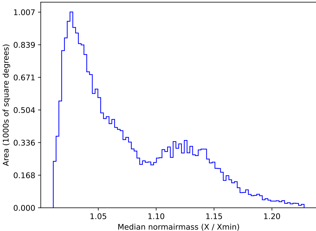
start_date_do90v3.4_10yrs All sky g band: Median normairmass
