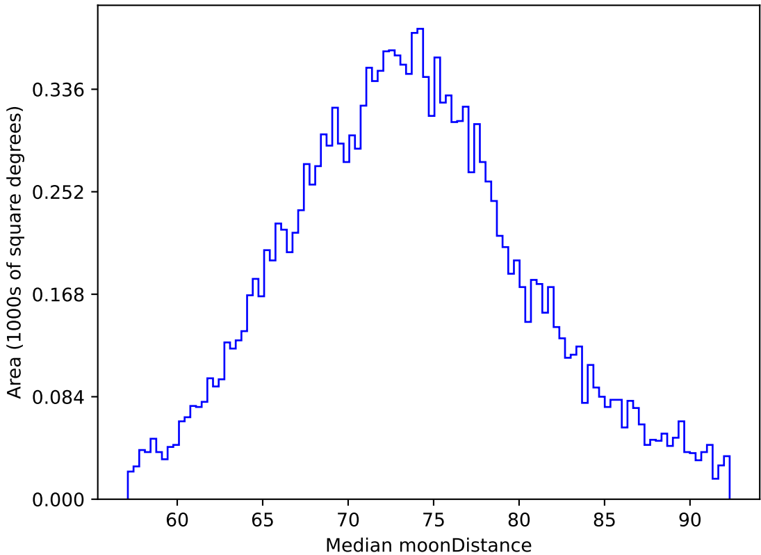
start_date_do90v3.4_10yrs WFD z band: Median moonDistance
