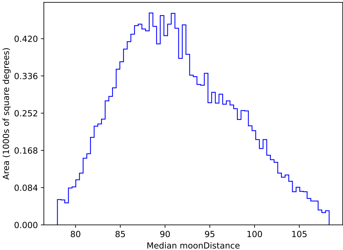
start_date_do90v3.4_10yrs WFD i band: Median moonDistance
