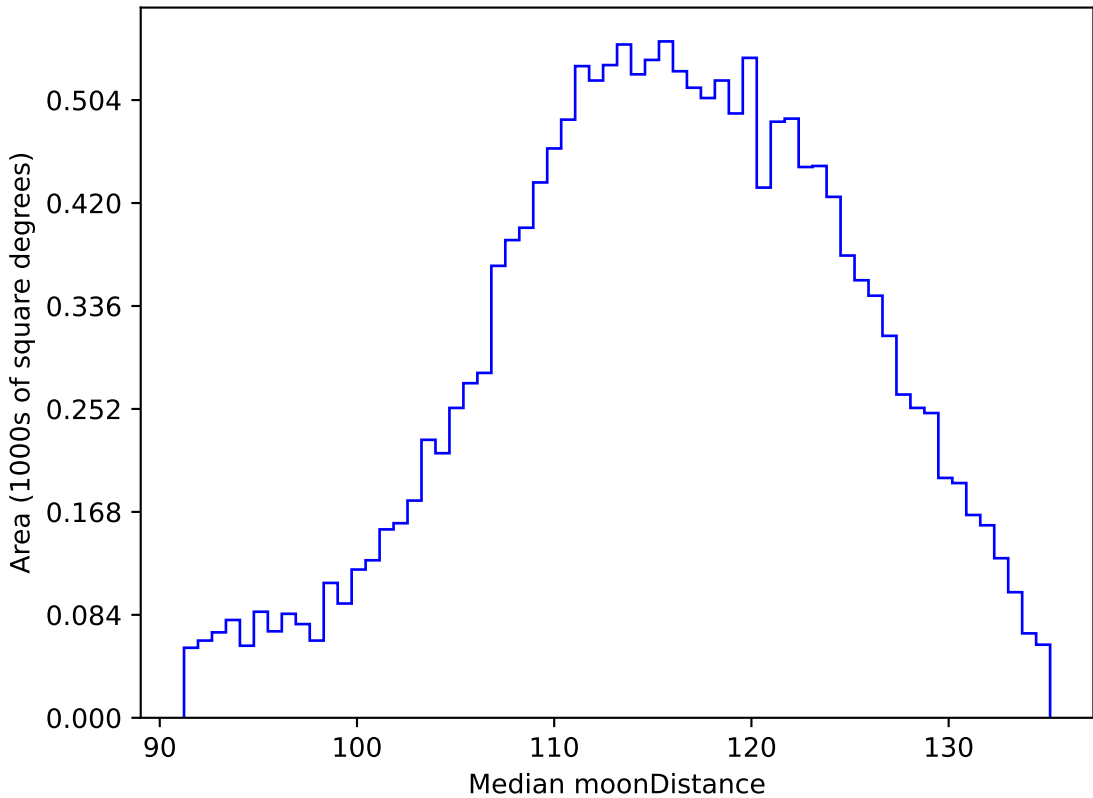
start_date_do90v3.4_10yrs WFD g band: Median moonDistance
