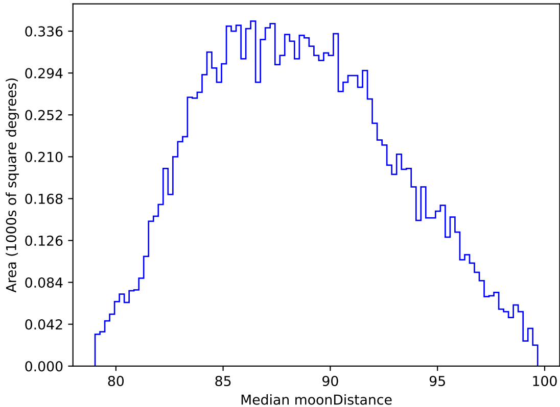
start_date_do90v3.4_10yrs WFD all bands: Median moonDistance
