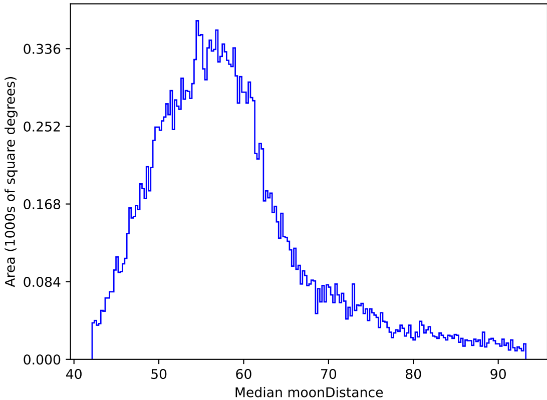
start_date_do90v3.4_10yrs All sky y band: Median moonDistance
