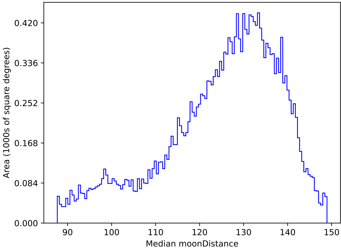
start_date_do90v3.4_10yrs All sky u band: Median moonDistance
