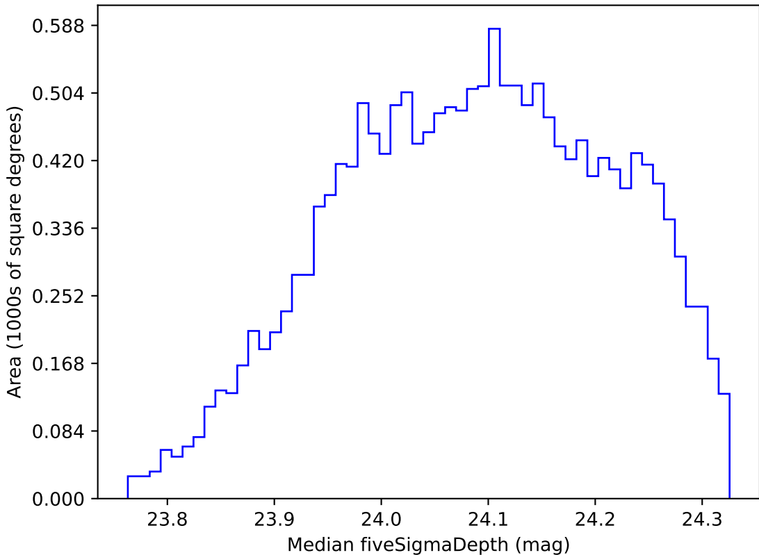
start_date_do90v3.4_10yrs WFD r band: Median fiveSigmaDepth
