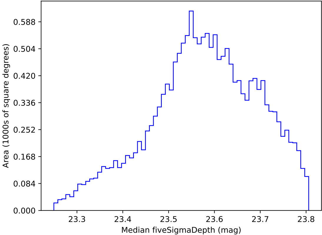
start_date_do90v3.4_10yrs WFD i band: Median fiveSigmaDepth
