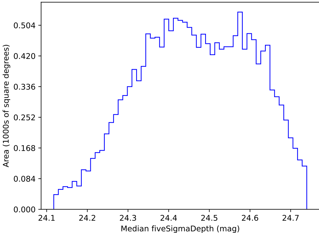
start_date_do90v3.4_10yrs WFD g band: Median fiveSigmaDepth
