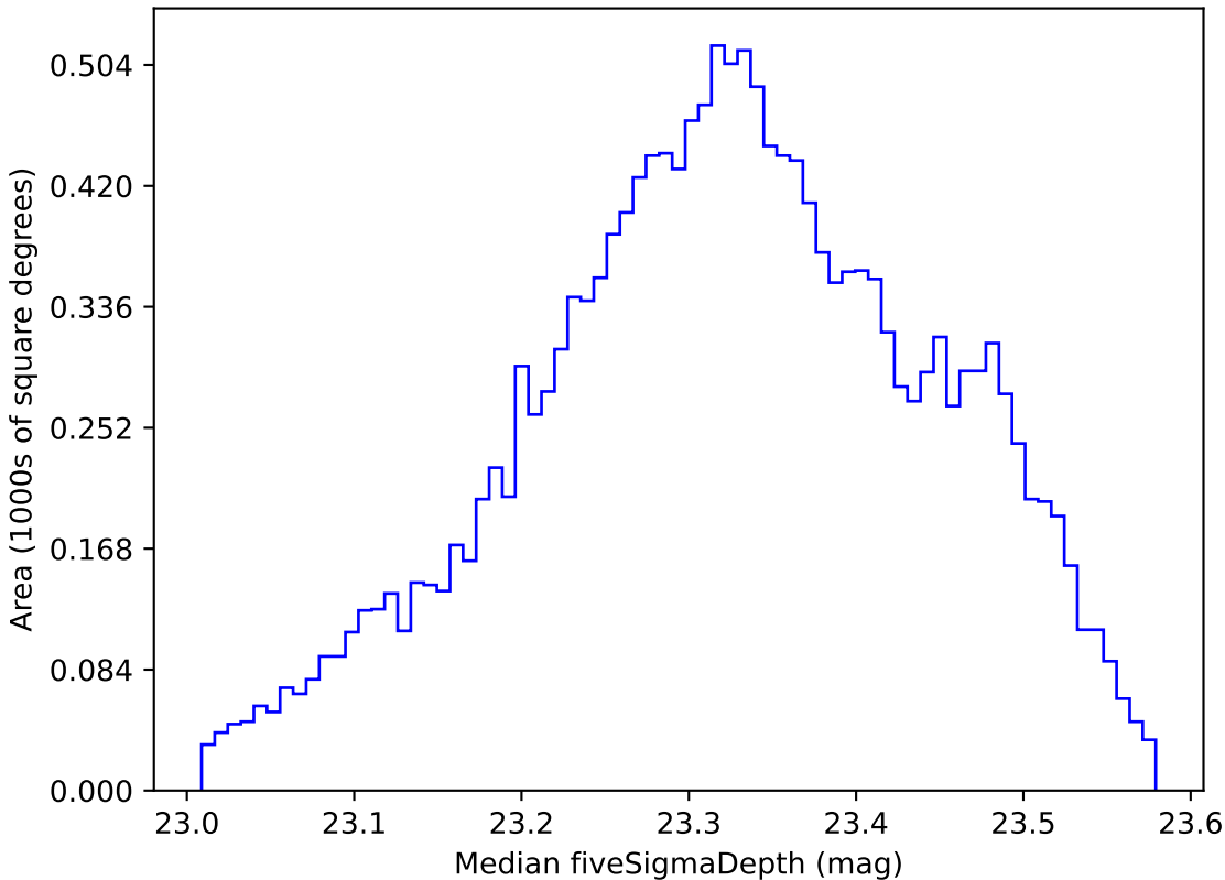
start_date_do90v3.4_10yrs WFD all bands: Median fiveSigmaDepth
