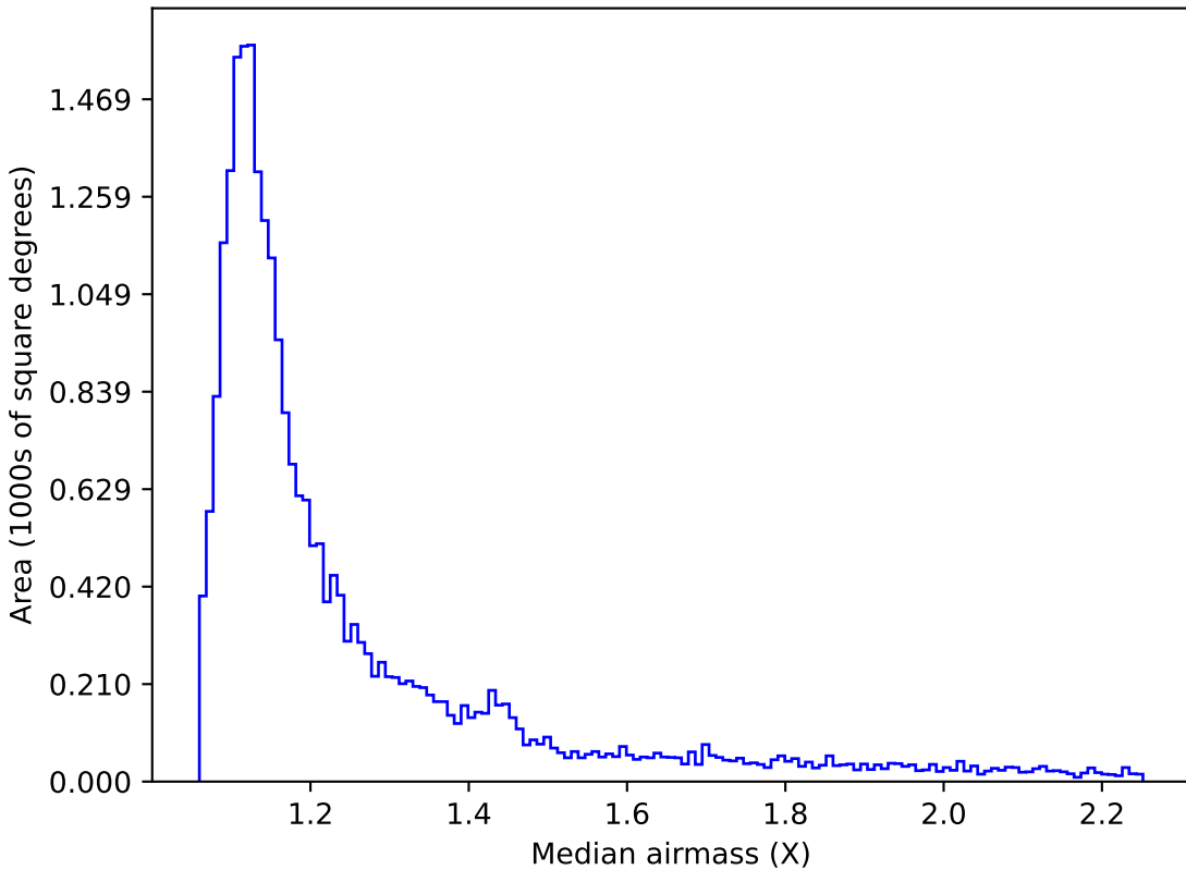
start_date_do90v3.4_10yrs Yr 1 z band: Median airmass
