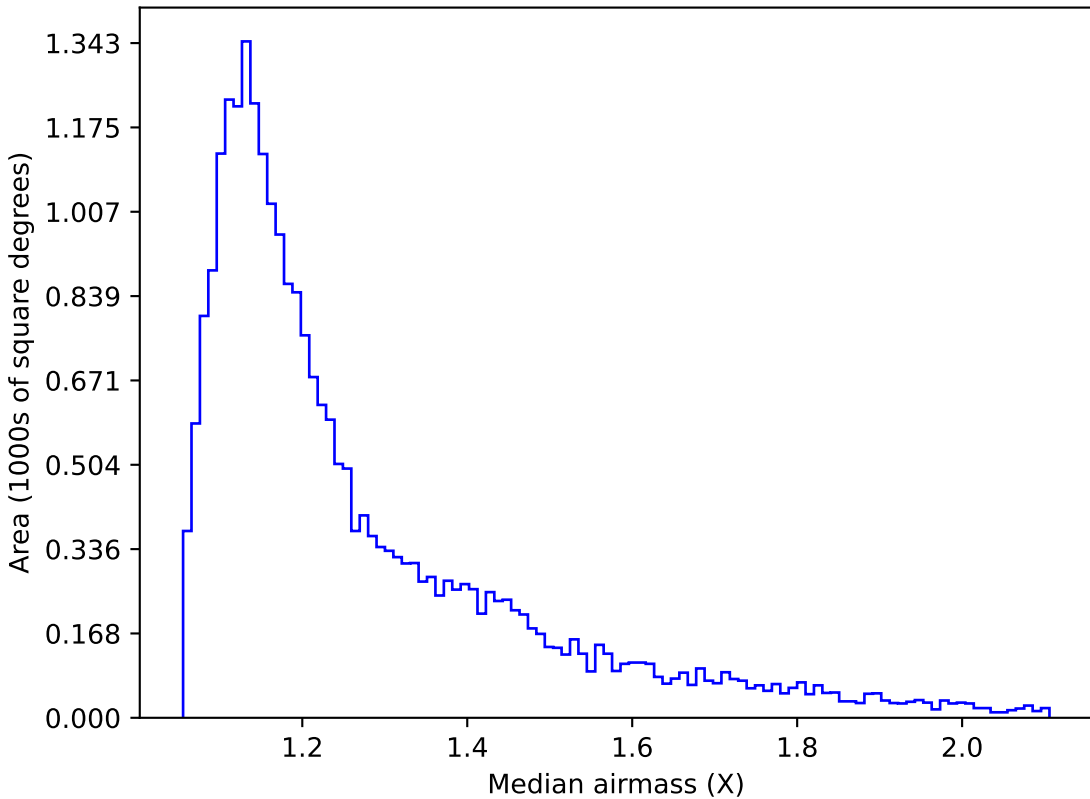
start_date_do90v3.4_10yrs Yr 1 g band: Median airmass
