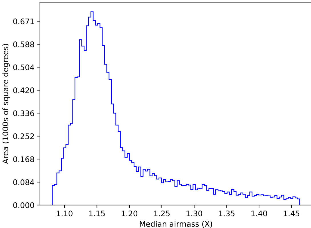
start_date_do90v3.4_10yrs WFD z band: Median airmass
