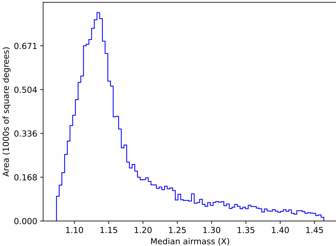
start_date_do90v3.4_10yrs WFD r band: Median airmass
