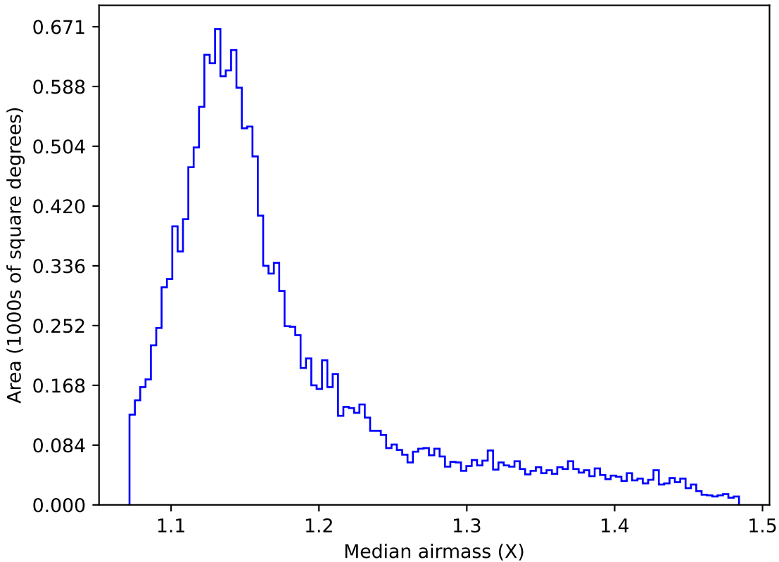
start_date_do90v3.4_10yrs WFD g band: Median airmass
