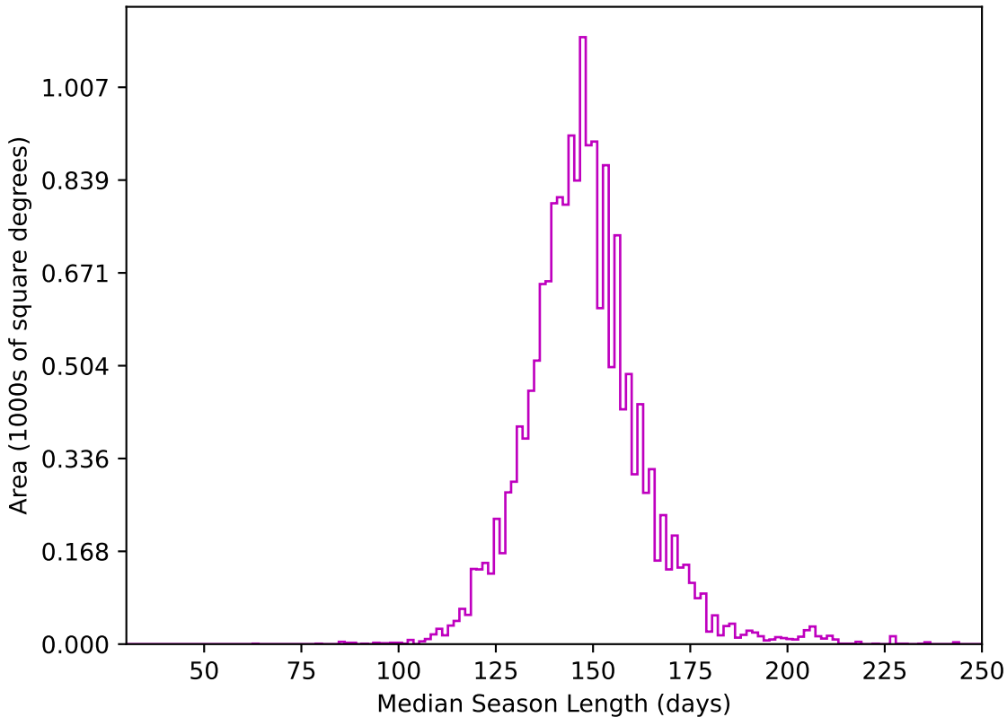
start_date_do90v3.4_10yrs WFD z band: Median Season Length
