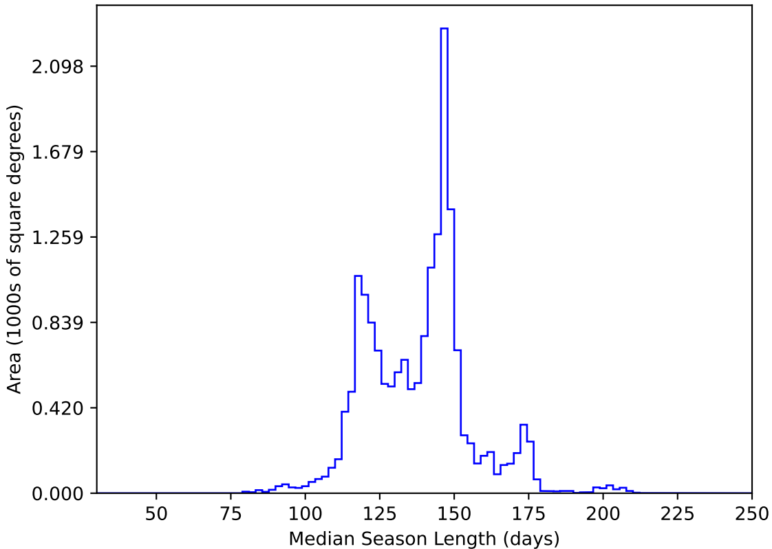
start_date_do90v3.4_10yrs WFD y band: Median Season Length
