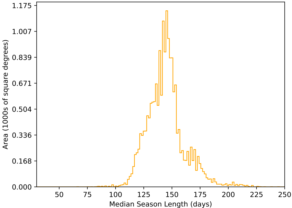
start_date_do90v3.4_10yrs WFD r band: Median Season Length
