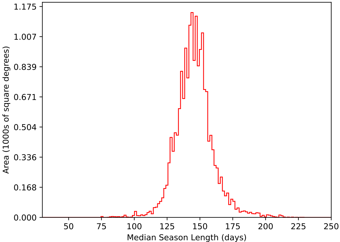
start_date_do90v3.4_10yrs WFD i band: Median Season Length
