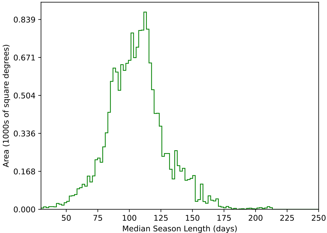
start_date_do90v3.4_10yrs WFD g band: Median Season Length
