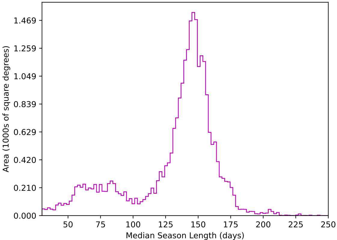
start_date_do90v3.4_10yrs All sky z band: Median Season Length
