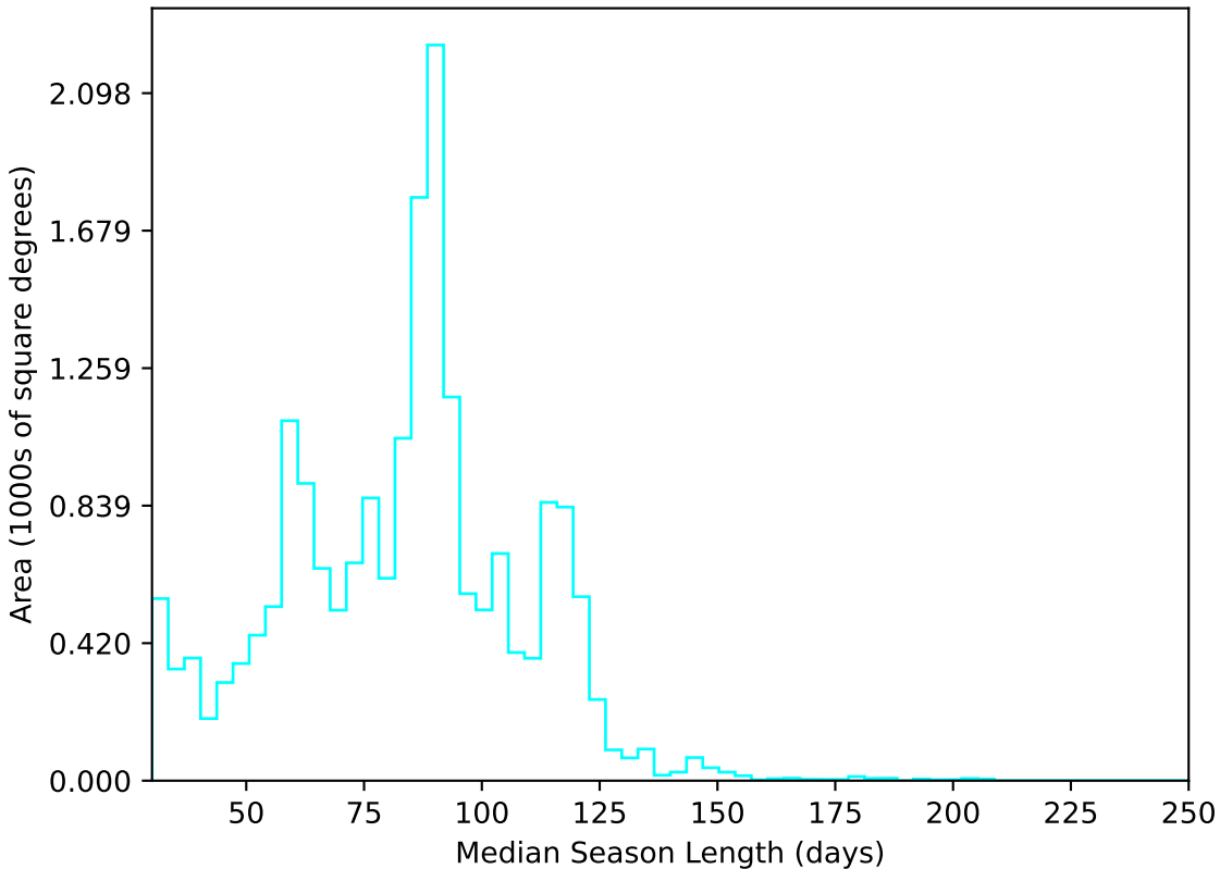
start_date_do90v3.4_10yrs All sky u band: Median Season Length
