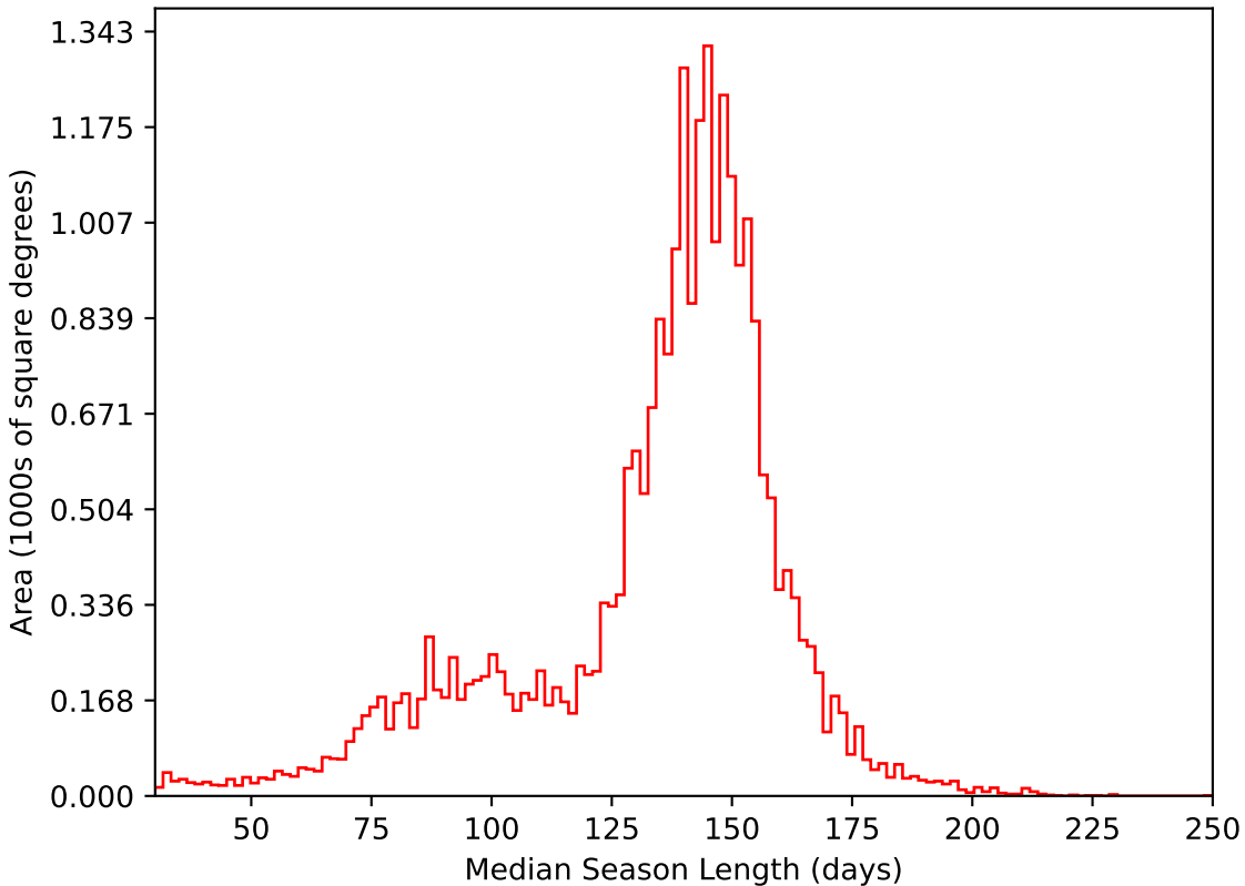
start_date_do90v3.4_10yrs All sky i band: Median Season Length
