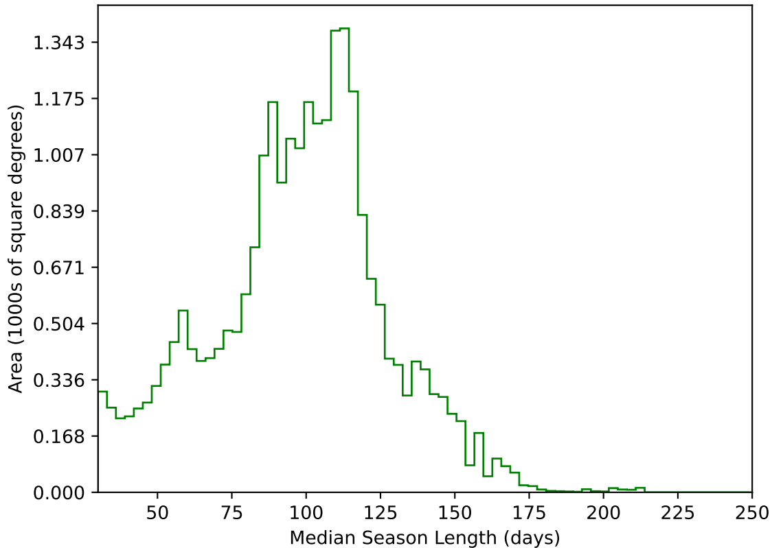
start_date_do90v3.4_10yrs All sky g band: Median Season Length
