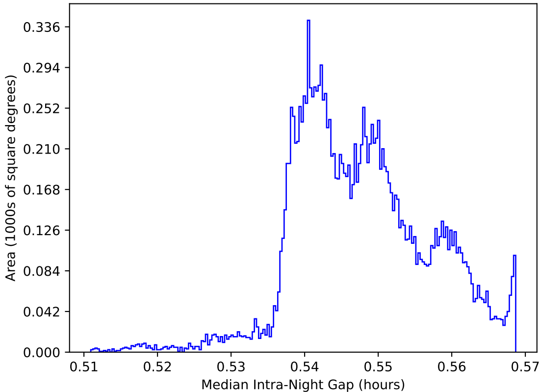
start_date_do90v3.4_10yrs WFD: Median Intra-Night Gap
