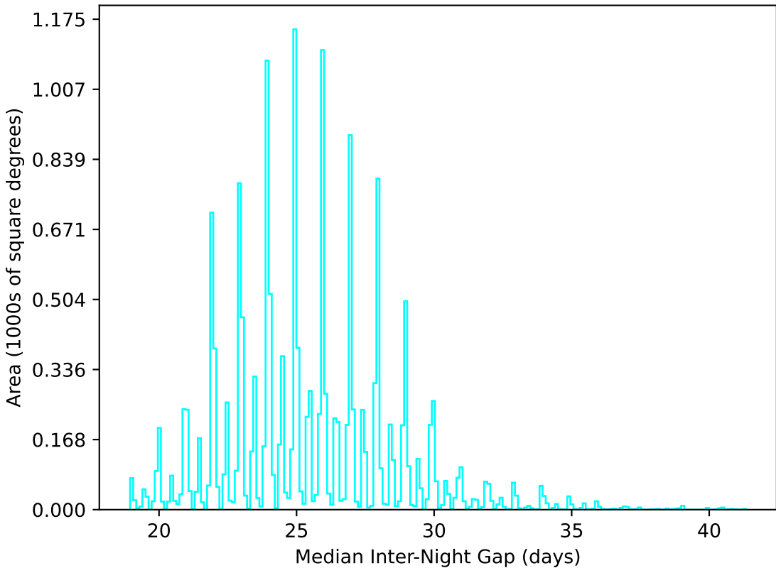
start_date_do90v3.4_10yrs WFD u band: Median Inter-Night Gap
