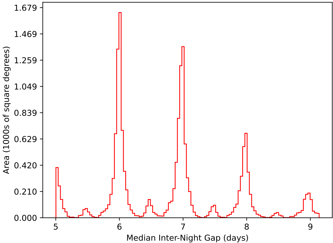
start_date_do90v3.4_10yrs WFD i band: Median Inter-Night Gap
