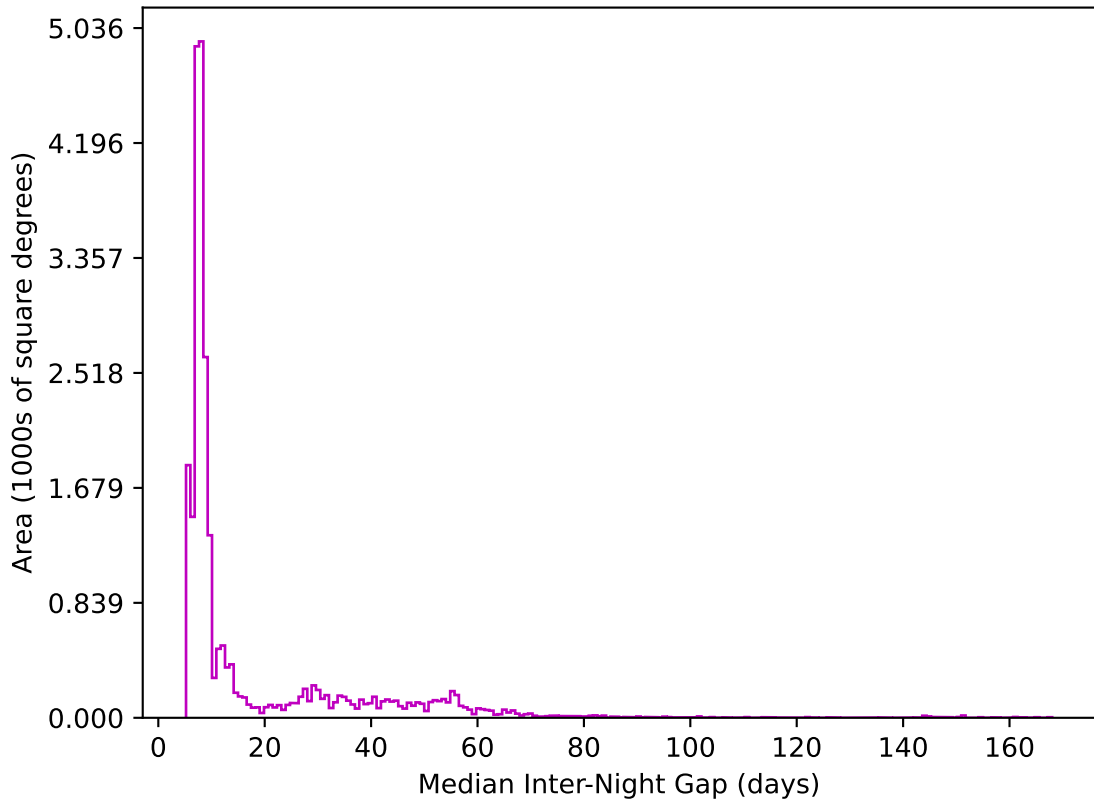
start_date_do90v3.4_10yrs All sky z band: Median Inter-Night Gap
