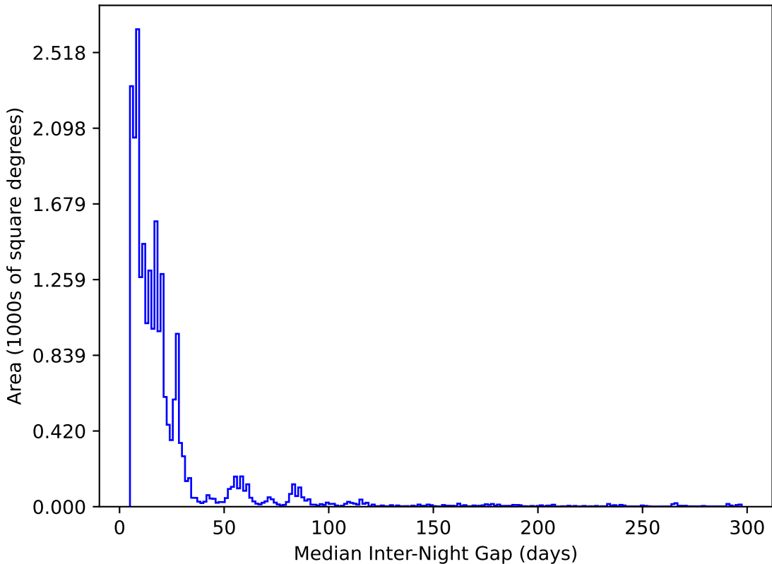
start_date_do90v3.4_10yrs All sky y band: Median Inter-Night Gap
