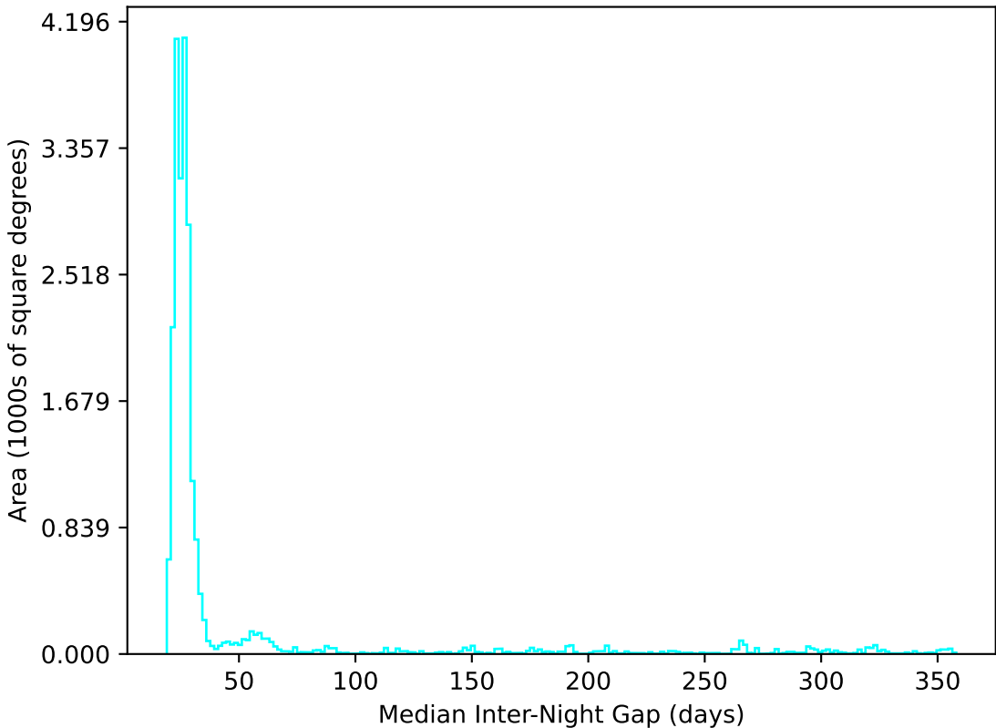
start_date_do90v3.4_10yrs All sky u band: Median Inter-Night Gap
