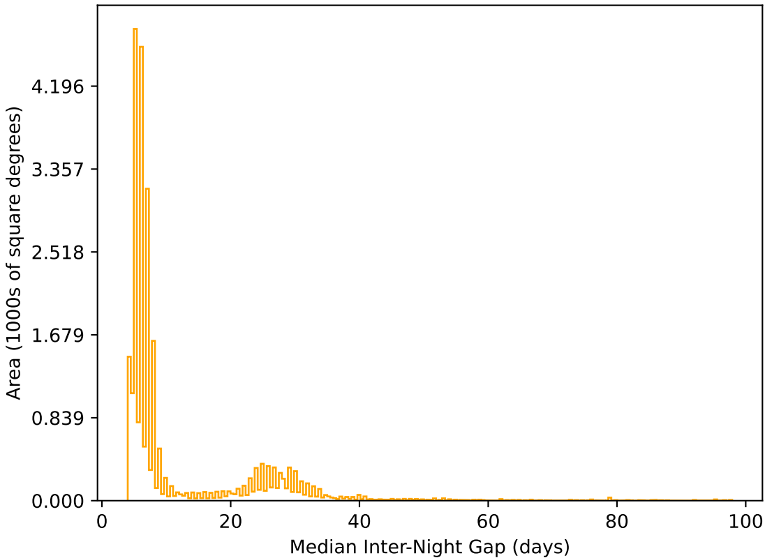
start_date_do90v3.4_10yrs All sky r band: Median Inter-Night Gap
